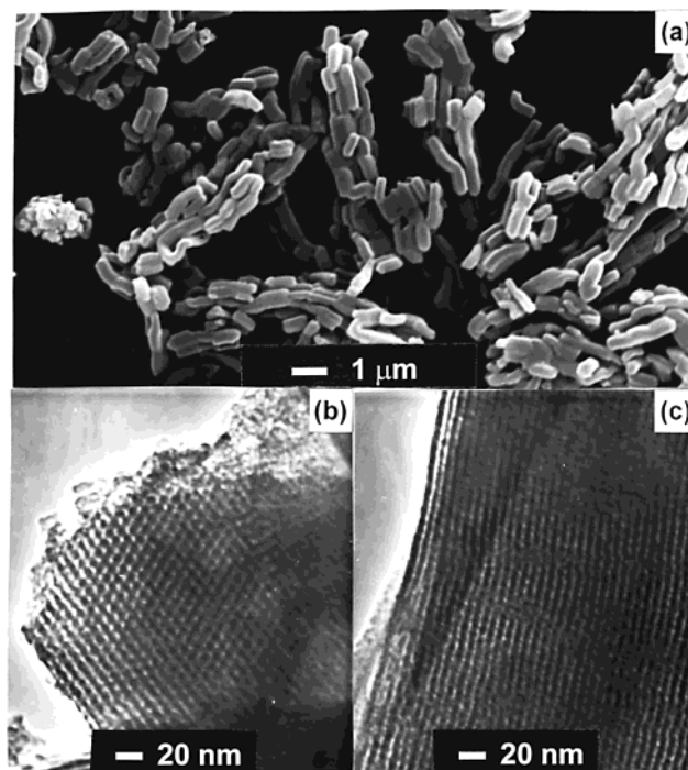
Figure 8. (a) SEM image and TEM images (b) in the direction of the pore axis and (c) in the direction perpendicular to the pore axis of an extracted sulfonic modified SBA-15 material (sample 9, Table 1).
