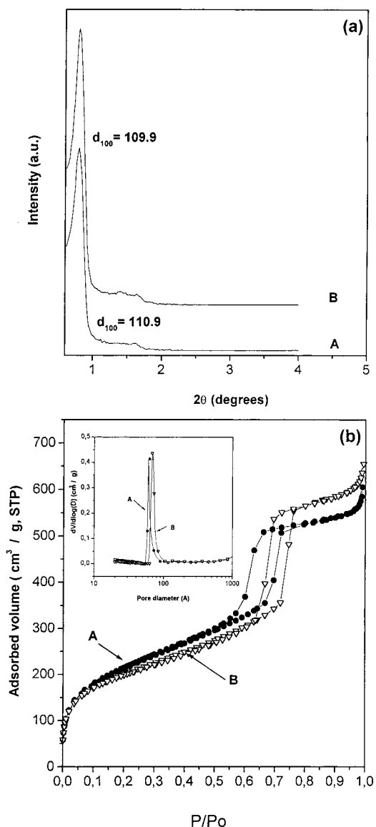
Figure 10. (a) XRD patterns of benzyl- and methylsulfonic-functionalized SBA-15 mesoporous materials after solvent extraction of the surfactant species. (b) N 2 adsorption/desorption isotherms and pore size distributions: (A) benzylsulfonic SBA-15 (●); (B) methylsulfonic SBA-15 (∇).
