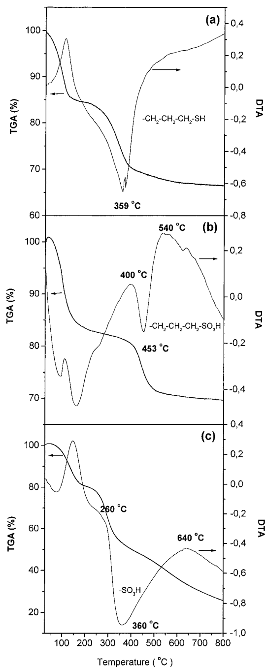
Figure 6. TGA and DTA measurements of different samples. (a) Thiol-functionalized mesoporous silica, sample 1 in Table 1. (b) Sulfonic-functionalized mesoporous silica obtained through the direct-synthesis approach, sample 8 in Table 1. (c) Sulfonic resin, Amberlyst-15.
