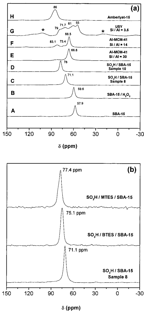
Figure 9. ^{31}\text{P} NMR spectra of TEPO chemically adsorbed (a) on conventional extracted SBA-15 (A), conventional extracted SBA-15 after treatment with aqueous \text{H}_2\text{O}_2 (30 wt %) at room temperature for 5 h (B), sulfonic-functionalized SBA-15 (C and D) and different conventional acid solids (E–H) and (b) on benzyl- and methylsulfonic-functionalized SBA-15 mesoporous materials.
