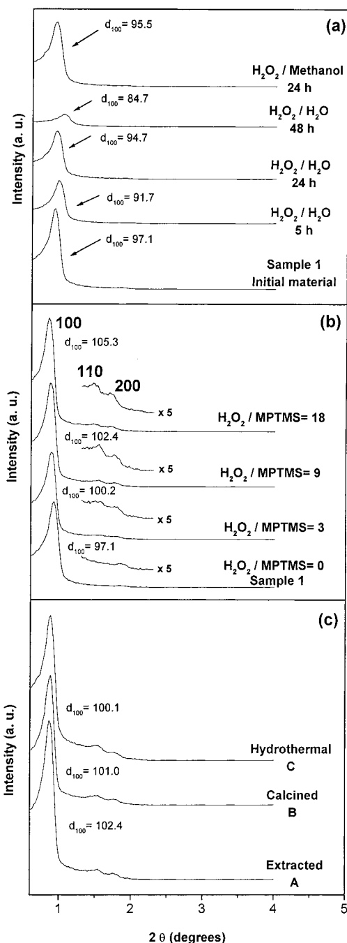
Figure 5. (a) XRD patterns of mercapto-modified samples after oxidation treatment in Ar atmosphere at different times and oxidant mixtures. (b) XRD patterns of different extracted functionalized mesoporous silicas synthesized in the presence of different H 2 O 2 /MPTMS molar ratios and using a MPTMS/(MPTMS + TEOS) molar ratio of 0.1 in the initial mixture. (c) XRD patterns of sulfonic-functionalized mesoporous silica after different treatments: (A) extraction with ethanol, sample 8 in Table 1; (B) as-made sample 8 after calcination in air, sample 11 in Table 2; (C) sample 8 after treatment in boiling water for 24 h.
