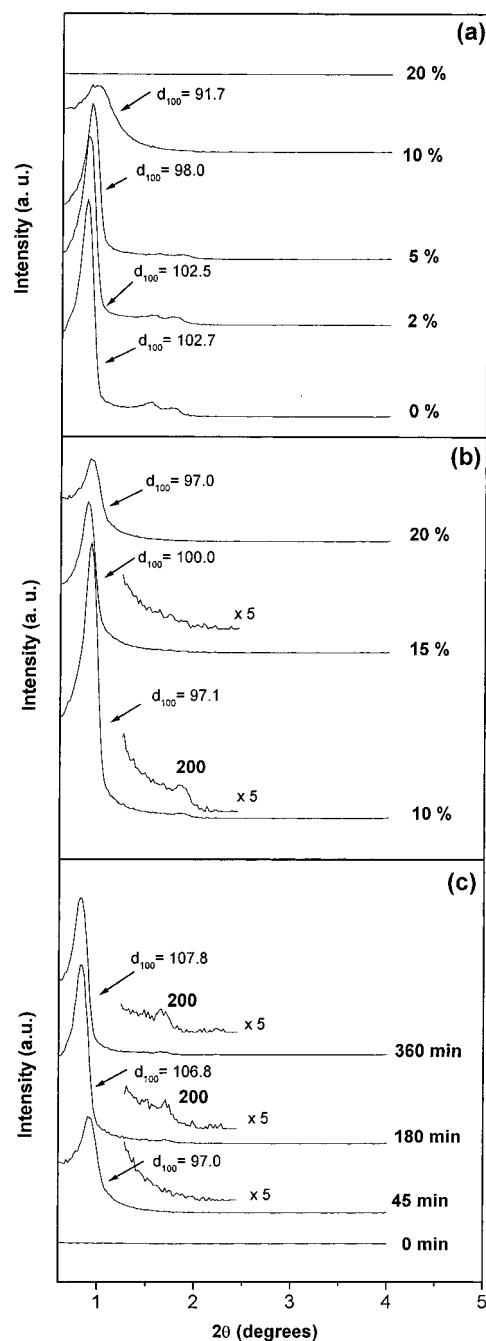
Figure 3. XRD patterns of extracted functionalized SBA-15 (a) with different molar ratios of MPTMS/(MPTMS + TEOS) in the initial mixture; (b) with different molar ratios of MPTMS/(MPTMS + TEOS) in the initial mixture and a TEOS prehydrolysis time of 45 min; (c) with MPTMS/(MPTMS + TEOS) = 0.2 in the initial mixture and different TEOS prehydrolysis times.
