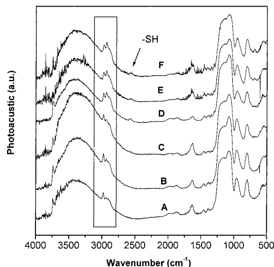
Figure 2. Photoacoustic infrared spectra of extracted functionalized SBA-15 synthesized with different molar ratios of MPTMS/(MPTMS + TEOS) in the initial mixture: (A) 0, (B) 0.02, (C) 0.05, (D) 0.10, (E) 0.15, and (F) 0.20.
