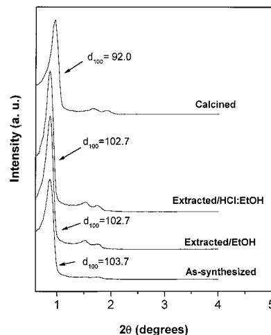
Figure 1. X-ray diffraction patterns obtained from conventional as-synthesized SBA-15 after different surfactant removal procedures.
