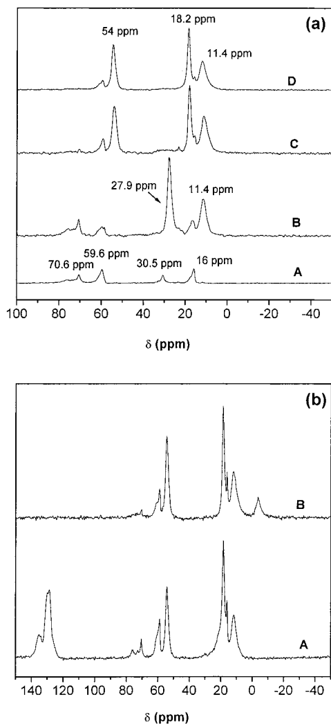
Figure 7. (a) CP MAS ^{13}\text{C} NMR spectra of different extracted SBA-15 mesoporous silicas: (A) conventional SBA-15; (B) thiol-functionalized SBA-15, sample 1 in Table 1; (C) sulfonic-functionalized SBA-15 obtained through the direct-synthesis approach, sample 8 in Table 1; (D) sulfonic-functionalized SBA-15 obtained through the direct-synthesis approach, sample 10 in Table 1 (b) CP MAS ^{13}\text{C} NMR spectra of bifunctionalized sulfonic mesoporous materials after extraction: (A) benzyl-sulfonic functionalized SBA-15; (B) methylsulfonic functionalized SBA-15.
