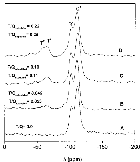
Figure 4. 29 Si NMR spectra of extracted functionalized SBA-15 synthesized with different molar ratios of MPTMS/(MPTMS + TEOS) in the initial mixture: (A) 0; (B) 0.05; (C) 0.1, TEOS prehydrolysis 45 min; and (D) 0.2, TEOS prehydrolysis 180 min. The measured relative integrated intensity ( T^m/Q^n ) of the organosiloxane ( T^m ) and siloxane ( Q^n ) NMR signals is depicted for each spectrum and compared to that expected from the composition of the initial mixture.
